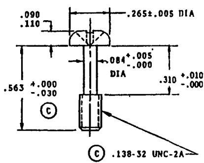
-9, -11 CAPTIVE SCREW, PHILLIPS HEAD
