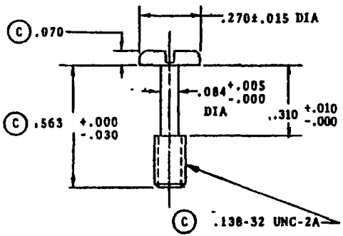
-4, -7 CAPTIVE SCREW, SLOTTED HEAD
