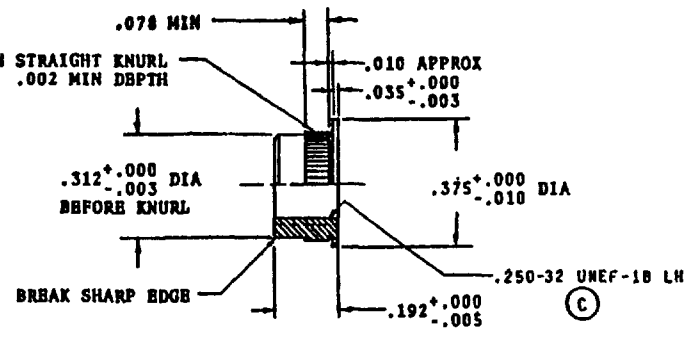
-2 COLLAR
